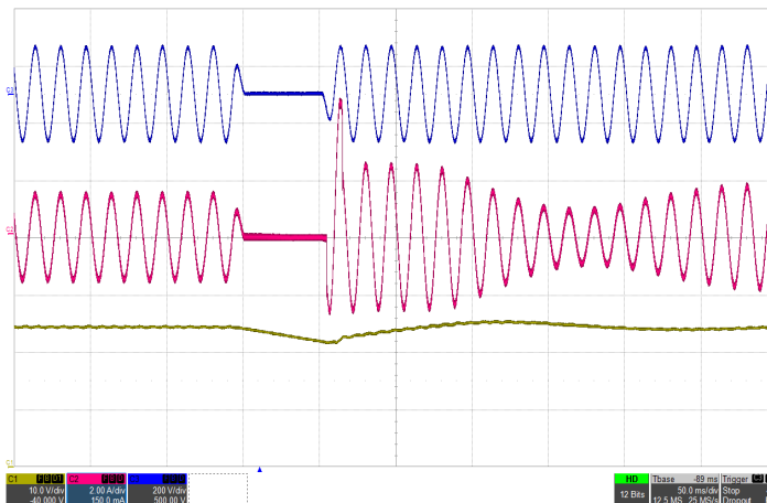
Figure 9: Line drop out with 400µF hold-up capacitor at full load current (115Vrms, 60Hz) Top: Vin (200V/div), Mid: Iin (2A/div), Bottom: Vout (10V/div), Timebase: (50ms/div).
