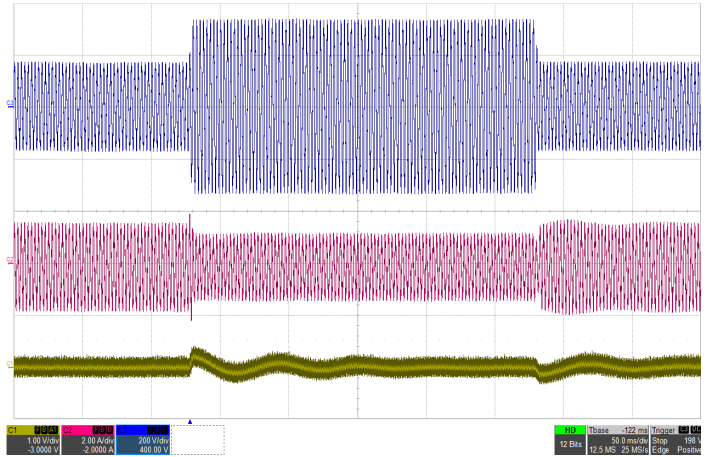
Figure 16: Input voltage transient response with 200µF hold-up capacitor at full load current (115Vrms-230Vrms-115Vrms, 400Hz), Top: Vin (200V/div), Mid: Iin (2A/div), Bottom: Vout (1V/div), Timebase: (50ms/div).
