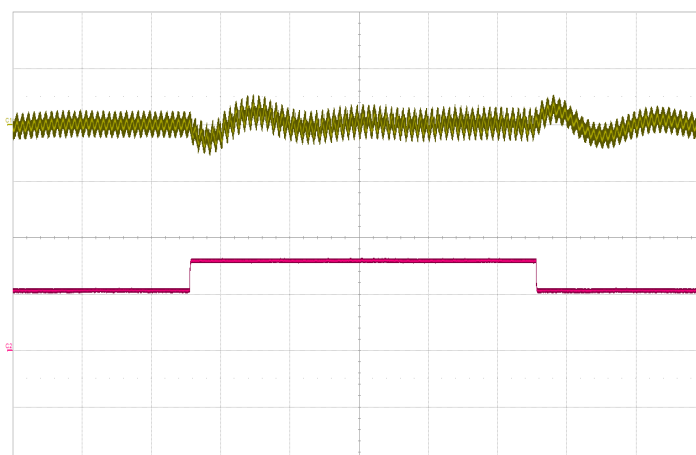
Figure 11: Regulated model output voltage response to step-change in load current with 200µF hold-up capacitor (50%-75%-50% of Iout(max), 115Vrms, 60Hz) Top: Vout (1V/div), Bottom: Iout (2A/div), Timebase: (100ms/div).
