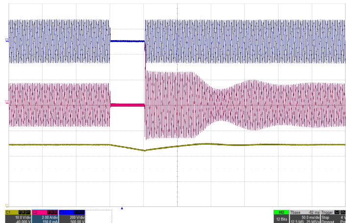
Figure 10: Line drop out with 400µF hold-up capacitor at full load current (115Vrms, 400Hz) Top: Vin (200V/div), Mid: Iin (2A/div), Bottom: Vout (10V/div), Timebase: (50ms/div).
