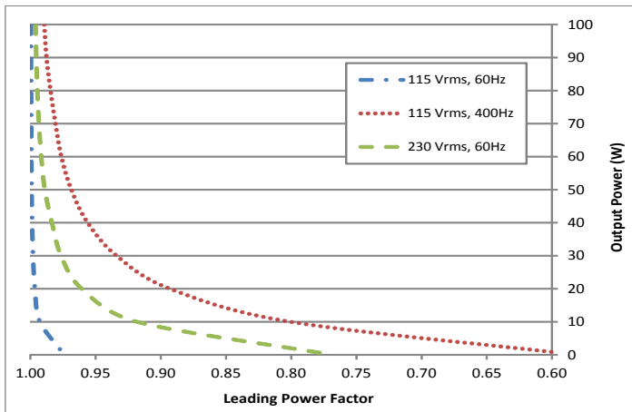
Figure 7: Output power vs. leading power factor (Tested with APFIC module and ACF-U-230-QM).
