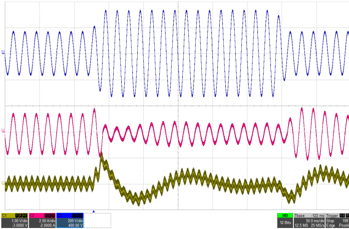
Figure 15: Input voltage transient response with 200µF hold-up capacitor at full load current (115Vrms-230Vrms-115Vrms, 60Hz), Top: Vin (200V/div), Mid: Iin (2A/div), Bottom: Vout (1V/div), Timebase: (50ms/div).
