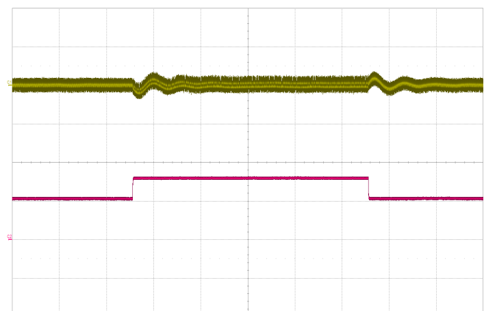
Figure 12: Regulated model output voltage response to step-change in load current with 200µF hold-up capacitor (50%-75%-50% of Iout(max), 115Vrms, 400Hz) Top: Vout (1V/div), Bottom: Iout (2A/div), Timebase: (100ms/div).
