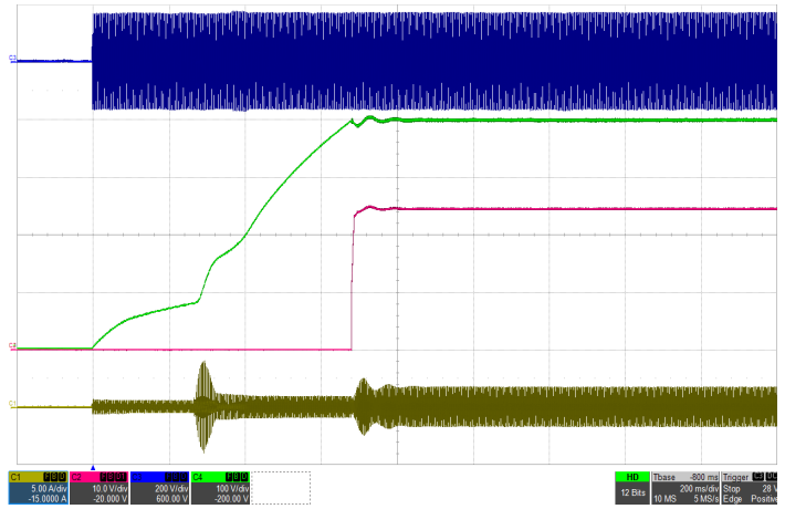
Figure 14: Typical startup waveform with 200µF hold-up capacitor (115Vrms, 400Hz) Top: Vin (200V/div), Top Middle: Hold-up capacitor voltage (100V/div), Bottom Middle: Vout (10V/div), Bottom: Iin (5A/div), Timebase: (200ms/div).
