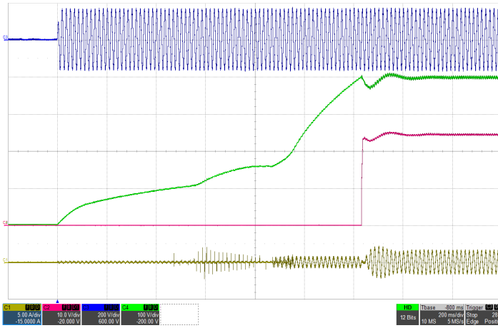
Figure 13: Typical startup waveform with 200µF hold-up capacitor (115Vrms, 60Hz) Top: Vin (200V/div), Top Middle: Hold-up capacitor voltage (100V/div), Bottom Middle: Vout (10V/div), Bottom: Iin (5A/div), Timebase: (200ms/div).
